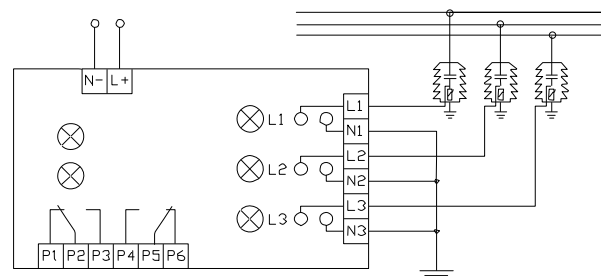
Wiring diagram of PBL
