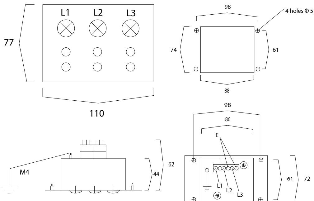
Dimensions of MCL-WS-01
