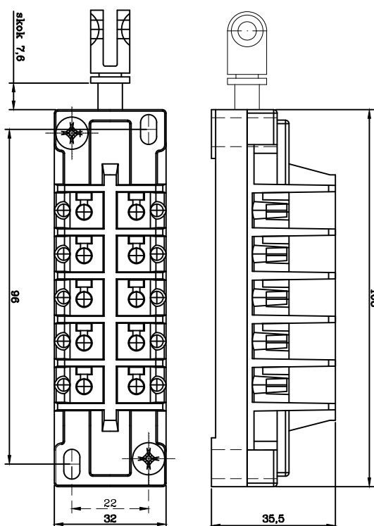
Dimensions of WK 5/10 limit switch
